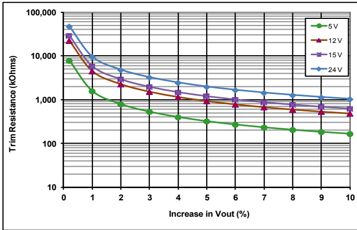
Common Figure 3: Trim graph for trim-up 5.0 to 24V outputs.
