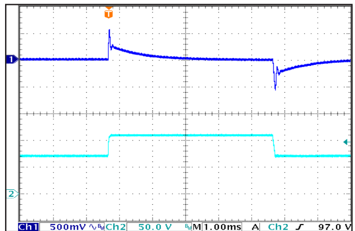
Figure 6: Output voltage response to step-change in input voltage (1000 V/ms, Vnom-Vmax-Vnom). Load cap: 1 μF ceramic capacitor. Ch 1: Vout, Ch 2: Vin.
