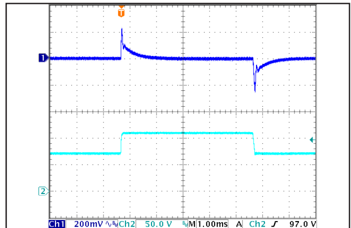
Figure 6: Output voltage response to step-change in input voltage (1000 V/ms, Vnom-Vmax-Vnom). Load cap: 1 μF ceramic and 15 μF tantalum capacitors. Ch 1: Vout, Ch 2: Vin.
